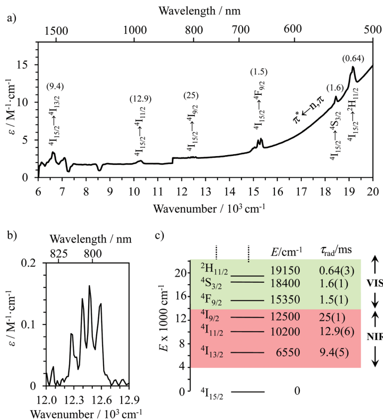
Fig. 6 (a) NIR-VIS absorption spectrum of [\text{GaErGa}(\text{bpb-bzimpy})_3]^{9+} (0.01 M in acetonitrile at 293 K) showing the \text{Er}(^{25+1}L_J \leftarrow ^4\text{I}_{15/2}) transitions and the associated radiative lifetimes (in ms) between parenthesis, (b) highlight of the \text{Er}(^4\text{I}_{9/2} \leftarrow ^4\text{I}_{15/2}) centered at 801 nm and (c) energy diagram of low-energy erbium-centered levels.
