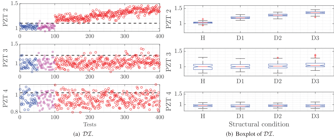
Figure 7. Damage index DI : (a) damage index DI : Healthy – training data (o), Healthy – test data( \square ) and Damaged (o). — is the threshold line assuming a significance level of 5%, (b) box plots to observe the median, quartiles and outliers in the index distribution. (a) DI . (b) Boxplot of DI .
