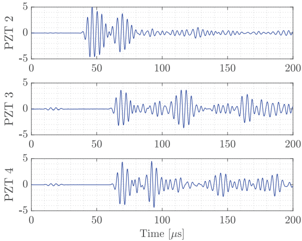
Figure 4. Healthy output time-series when PZT 1 acts as an actuator with a central frequency of 250 kHz. Please refer to the online version of the article to view the figure(s) in color.
