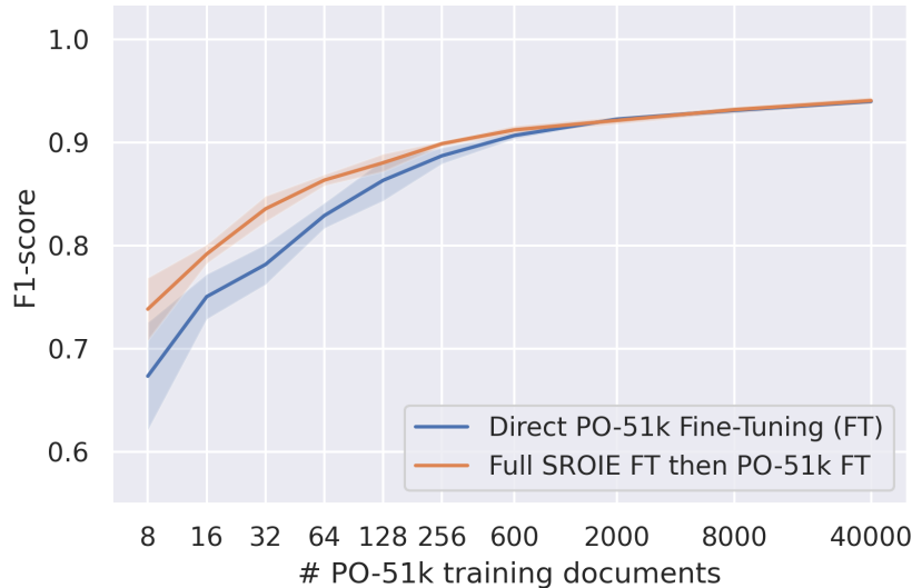
Fig. 5: Test F1 scores of pre-trained LayoutLM when transferring extraction knowledge from SROIE to PO-51k tasks. The IE performance is always improved by resorting to SROIE as an intermediate task, the boost being significant with few available PO-51k documents for fine-tuning.
