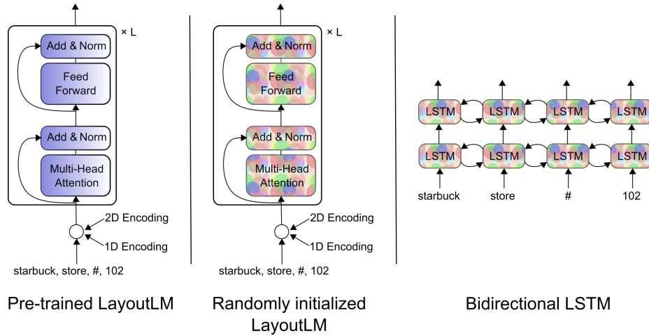
Fig. 1: The different architectures used in our experiments for encoding documents. From left to right: Transformer-based LayoutLM [36] with pre-trained weights, LayoutLM with random initialization and a 2-layer bidirectional LSTM also randomly initialized.
