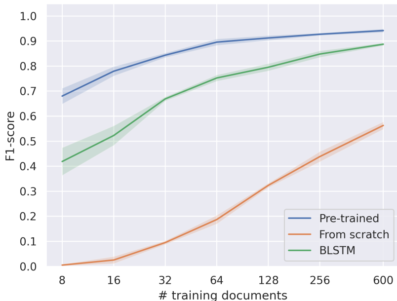
Fig. 3: Few-shot extraction performance on the SROIE [16] test set for the pre-trained LayoutLM [36] against its randomly initialized version and a BLSTM network.
