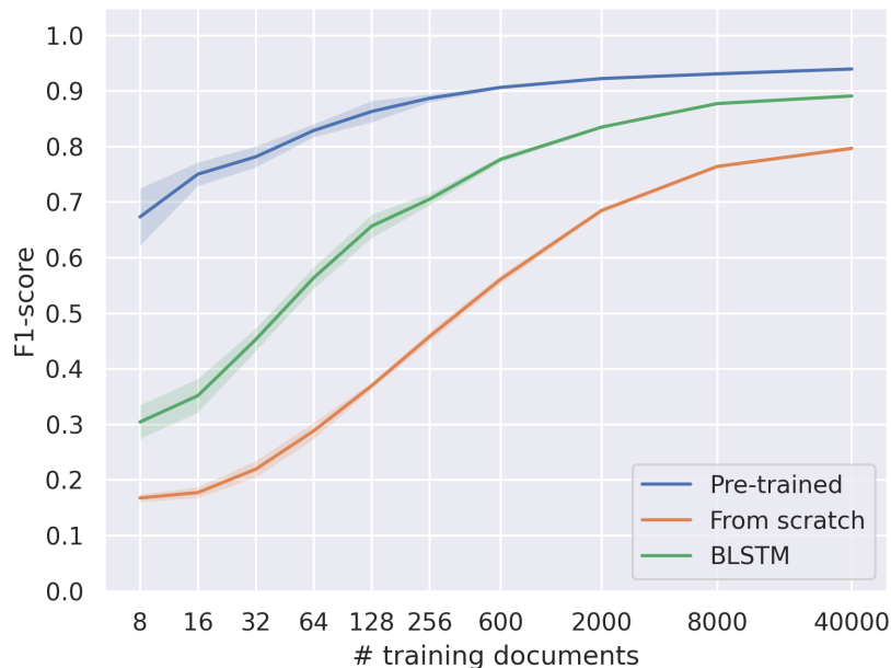
Fig. 4: Few-shot extraction performance on the PO-51K test set for the pre-trained LayoutLM [36] against its randomly initialized version and a BLSTM network.
