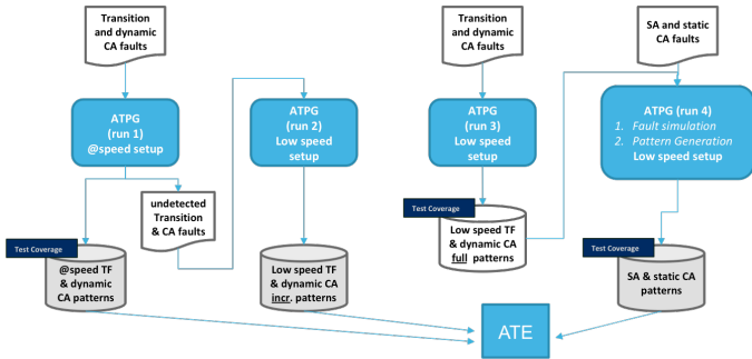
Figure 2: Example of a multi-run industrial ATPG flow
