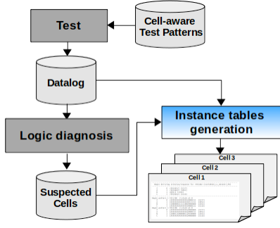
Figure 7: Generation flow of instance tables
