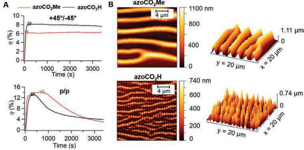
Figure 4. A) Time evolution of the first-order diffraction efficiency \eta of \text{azoCO}_2\text{Me} (red curve) and \text{azoCO}_2\text{H} (black curve) thin films subjected to +45^\circ/-45^\circ (top) and p/p (bottom) interferential illumination at 488 nm ( 240 \text{ mW cm}^{-2} each beam). Diffraction efficiency maxima are indicated by empty squares. B) AFM imaging (2D and 3D views) of \text{azoCO}_2\text{Me} and \text{azoCO}_2\text{H} thin films after p/p interferential illumination at 488 nm for 1 h ( 240 \text{ mW cm}^{-2} each beam).
