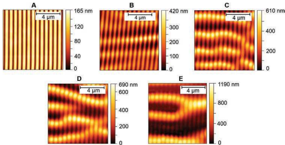
Figure 5. AFM imaging of \text{azoCO}_2\text{Me} thin film subjected to interferential illumination at 488 nm with a p/p polarization configuration ( 240 \text{ mW cm}^{-2} each beam, \Lambda = 0.74 \mu\text{m} ) after irradiation for: A) 2, B) 8, C) 15, D) 30, and E) 60 min.
