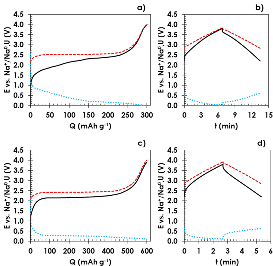
Figure 4: Pre-sodiation of a negative electrode (a) hard carbon, and (c) tin phosphide in an NIC with NaBH 4 /AC-positive electrode. Galvanostatic profiles of the composite-positive electrode (red dashed line), -negative electrode (blue dotted line), and voltage of the cell (black solid line). Galvanostatic charge/discharge profiles of NIC with (b) HC-negative electrode at 125 \text{ mA g}^{-1} and with (d) SnP-negative electrode at 250 \text{ mA g}^{-1} (values given per gram of the total mass of the electrodes) in the voltage range 2.2–3.8 V.
