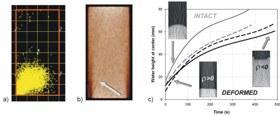
Figure 4. Mechanical and capillary imbibition data for sample BNT#2. (a) Location of acoustic emissions in a central cross-section. (b) Raw image of a scan in the central cross-section: the arrow shows the presence of an incipient fracture. (c) Comparison of the water heights evolution in the intact (grey) and deformed (black) samples. Solid curves are the fitting curves for central height, dashed curves are for fitting curves for the border height.
