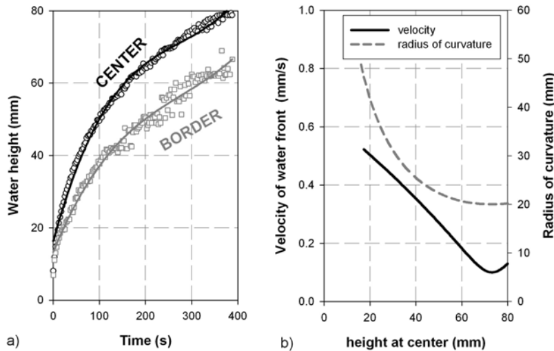
Figure 2. Measured parameters for an intact Bentheim sandstone sample. (a) Water height in the center (black) and on the border (grey) vs. time. Symbols are for measurements on the images, lines are for fitting curves (third power polynomial function). (b) Velocity (solid black) and radius of curvature (dashed grey) vs. height at center.
