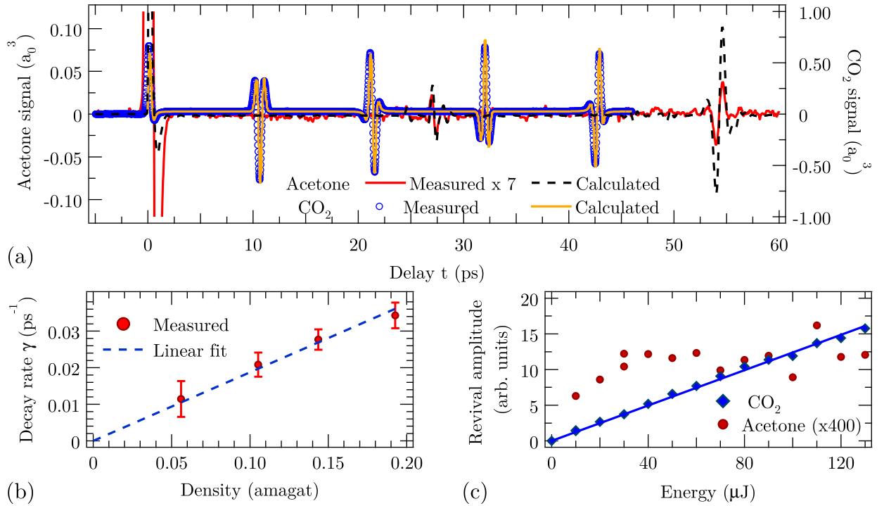
FIG. 4. (a) Alignment signal recorded in 0.15 bar of room-temperature acetone (red solid line) and CO 2 (blue circles) molecules induced by a linearly polarized laser pulse ( \mathcal{P}_1 ) of intensity 12 TW/cm 2 , and the corresponding quantum simulations for acetone (black dashed line) and CO 2 (yellow solid line) performed in collision-free conditions using Eq. (2). The vertical scales are given in Bohr units and the acetone signal is magnified by a factor 7 to help the eyes. (b) Collisional decay rate constant of the alignment revivals of acetone (red solid circles) as a function of the gas density expressed in amagat (1 amagat \equiv 2.69 \times 10^{25} molecules/m 3 ) with error bars representing one standard deviation. The density normalized decay time constant is obtained from the linear fit applied to the data (blue dashed line). (c) Laser energy dependence of the peak amplitude of the revival of CO 2 (blue diamonds) and acetone (red solid circles) measured under the same experimental conditions (0.15 bar). Linear fit of the CO 2 data (blue solid line).
