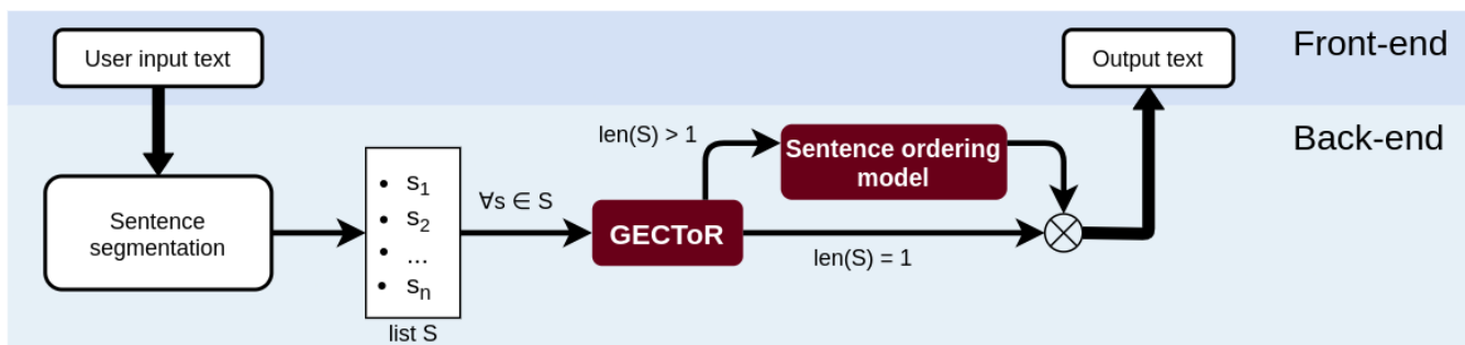
FIGURE 1 – GECKo+'s pipeline.
