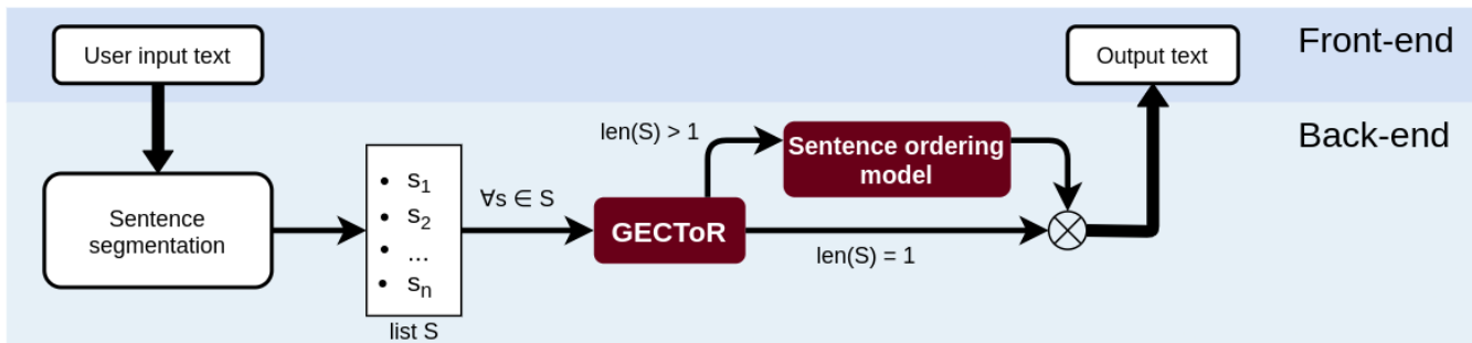
FIGURE 1 – GECKo+'s pipeline.
