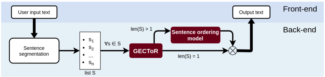
FIGURE 1 – GECKo+'s pipeline.
