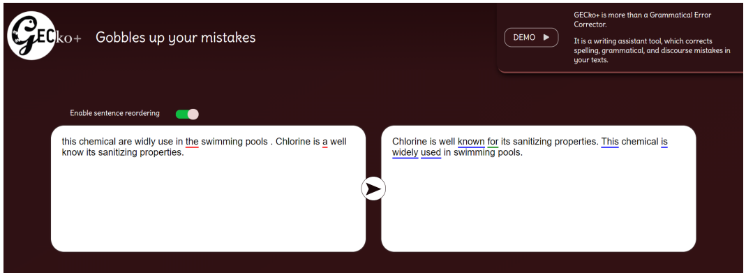
FIGURE 2 – GECKo+'s interface.
