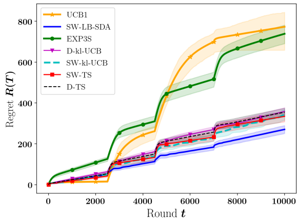
Figure 5. Performance on a Gaussian instance with a constant standard deviation of \sigma = 0.5 averaged on 2000 independent runs.
