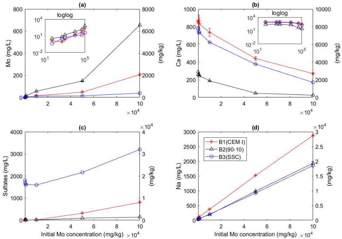
283 Figure 1 – Experimental leached element concentrations (expressed in mg/L on the y-axis at left and 284 in \text{mg}_{\text{Mo}}/\text{kg}_{\text{binder}} on the y-axis at right) plotted as a function of the initial Mo spike in the binders 285 expressed in \text{mg}_{\text{Mo}}/\text{kg}_{\text{binder}} . All values are related by lines for ease of reading and are presented in a 286 linear scale. Mo and Ca data are also plotted in logarithmic scale to analyze trends at low Mo 287 concentrations. (a) Molybdenum, (b) calcium, (c) sulfates, (d) sodium. Two solution samples were 288 analyzed per formulation and arithmetic mean values are presented with a confidence interval of 95%.
