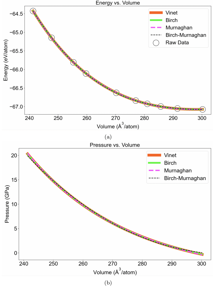
Figure 3: The fitted equation of state (EOS) plots for (a) Energy vs. Volume and (b) Pressure vs. Volume data obtained by differentiating the energy with a central difference scheme using different EOS models. Here, the material under investigation is T_d - \text{MoTe}_2 for which ‘Energy vs. Volume’ data was computed using the VASP code (numerical details are given in Ref. [105]).
