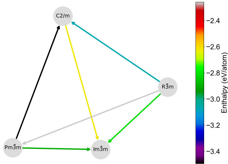
Figure 7: A network plot of the phase transition paths for different phases of Bi. The color of the arrows represents the relative enthalpy for different phase transitions.
