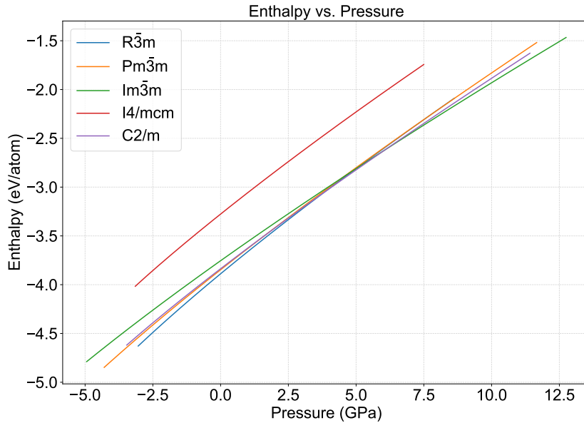
Figure 5: Enthalpy variation with pressure for five different phases of Bi as calculated using the plot_enthalpy_curves function.
