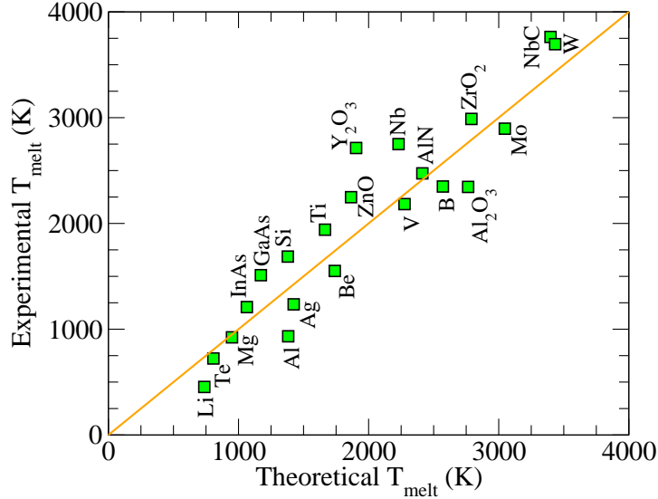
Figure 1: A comparison of the theoretically estimated (using Eq. 46) and experimentally reported melting temperature ( T_{melt} ) data for some elemental and binary compounds. All the structures and their elastic-tensor data were obtained from the Materials Project database [22], and the experimental data were obtained from the website: https://www.americanelements.com/ . The mp ID of the structures is as follows: Li (mp-135), Te (mp-19), Mg (mp-153), InAs (mp-20305), GaAs (mp-2534), Si (mp-149), Al (mp-134), Ag (mp-124), Ti (mp-46), Be (mp-87), ZnO (mp-2133), Y_2O_3 (mp-2652), Nb (mp-75), V (mp-146), AlN (mp-661), B (mp-160), Al_2O_3 (mp-1143), ZrO_2 (mp-1565), Mo (mp-129), NbC (mp-910), and W (mp-91).
