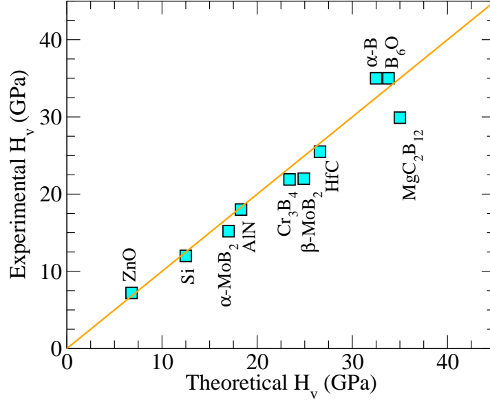
Figure 2: A comparison of the available experimental Vickers hardness ( H_v ) data with the theoretical values obtained using the recommended model in Section 5.1 for several materials listed in Table 2.
