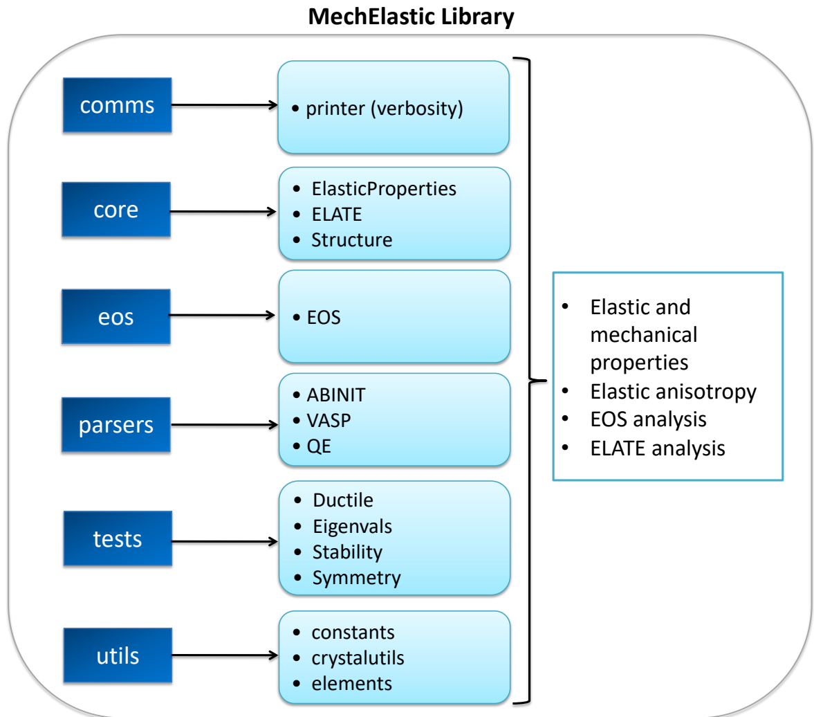
Figure 8: A structural overview of the MECHELASTIC library
