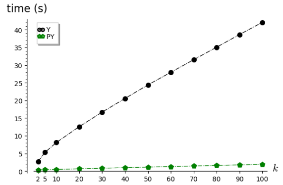
(b) Average running time on Switzerland
