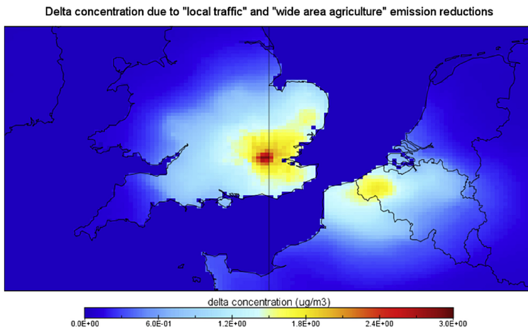
Fig. 7. Delta PM 2.5 concentrations (µg/m 3 ) obtained with SHERPA for a scenario focusing on local traffic emission reductions and agricultural emission reductions over a wider area including parts of neighbouring countries.
