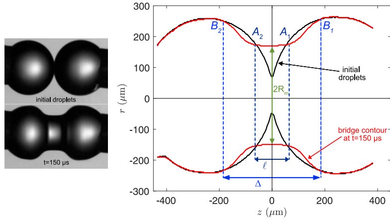
FIG. 3. Shadow images (left) and detected contour (right) of the initial drops and the bridge at t=150 \mu\text{s} , in the case of two water drops of the same radius, R=250 \mu\text{m} . The vertical dashed lines passing by points B_1 and B_2 correspond to the limits of the bridge. The vertical dashed lines passing by points A_1 and A_2 correspond to the limit of the cylindrical part of the bridge, which is present in the inertial regime.
