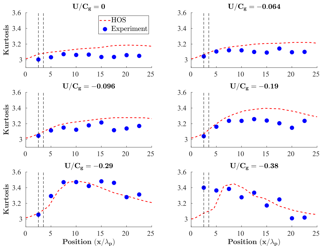
FIG. 11. Spatial evolution of the kurtosis along the wave flume for different current velocities. Comparison between experiments and numerical simulations.
