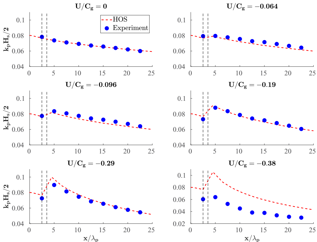
FIG. 9. Evolution of local steepness, k_p H_s / 2 , during wave propagation. Comparison between experiments and numerical simulations.
