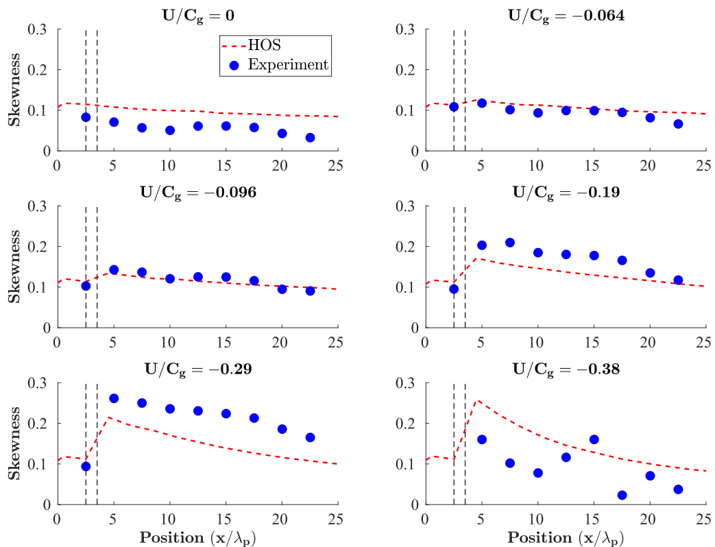
FIG. 10. Spatial evolution of the skewness along the wave flume for different current velocities. Comparison between experiments and numerical simulations.
