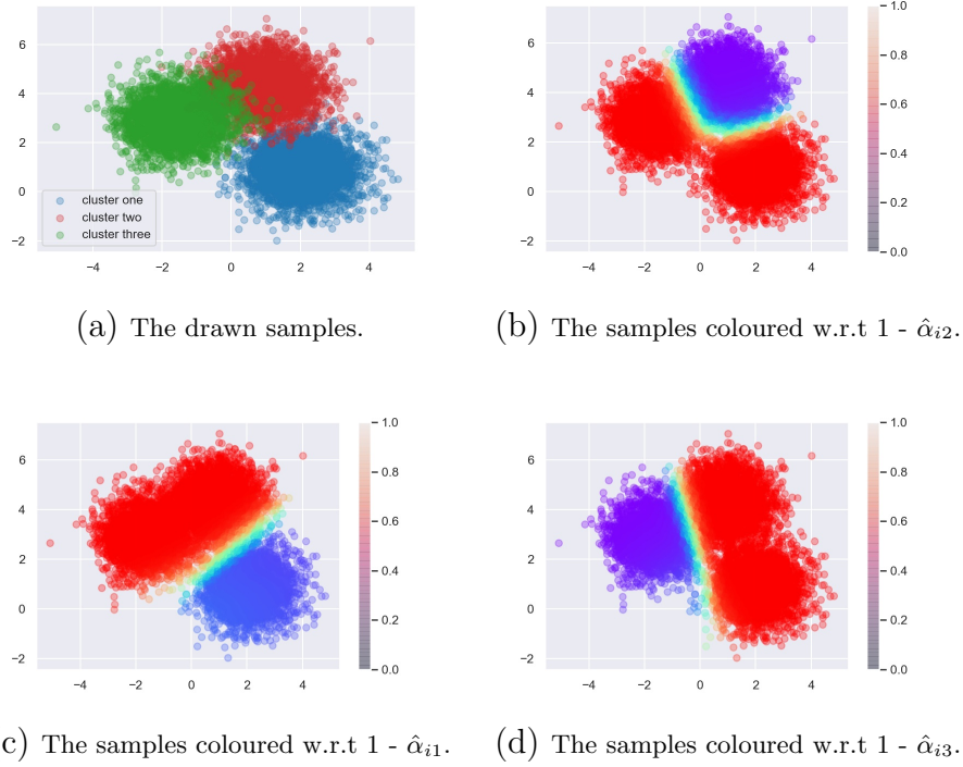
Figure 9: Three clusters generated using the make_blobs function of scikit-learn package as well as their reproduced clustering performed by DPWTE ( \tilde{p} = 3 ).
