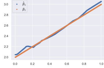
(a) DPWTE: \hat{\beta}_1 vs \beta_1
