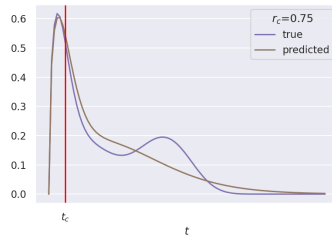
(g) r_c = 0.75, \tilde{p} = 2
