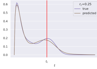
(c) r_c = 0.25, \tilde{p} = 3
