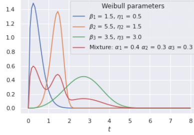
Figure 13: Densities of \mathcal{W}_3^3 and its composing distributions.
