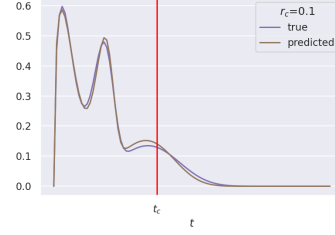
(b) r_c = 0.1, \tilde{p} = 3
