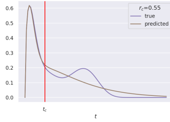
(e) r_c = 0.55, \tilde{p} = 2
