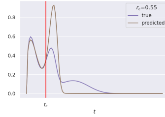
(f) r_c = 0.55, \tilde{p} = 2
