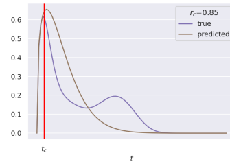
(h) r_c = 0.85, \tilde{p} = 1
