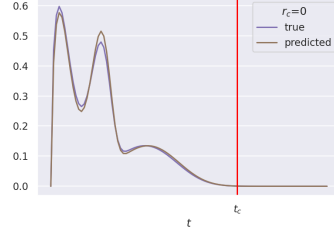
(a) r_c = 0, \tilde{p} = 3
