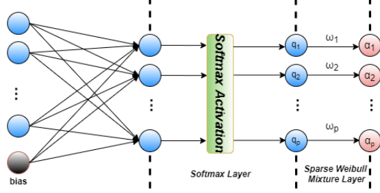
Figure 4: Softmax and Sparse Weibull Mixture layers of clf
