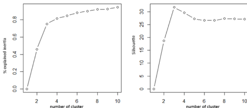
Figure 7. Silhouette Values to define the optimum of cluster .
