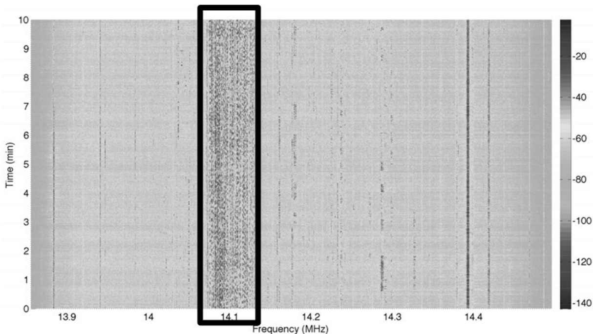
Figure 9.7: HFSA_IDeTIC_F1_V01 database extraction for HF channel traffic during a radio-ham contest at 14.1 MHz (area highlighted in the rectangle) [48].
