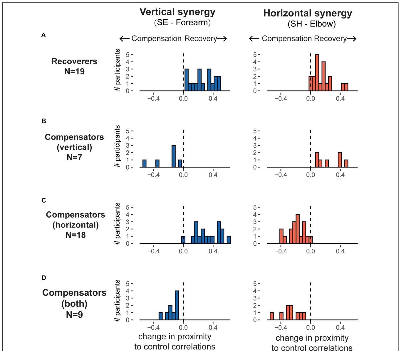
FIGURE 6 | Histograms of evolution of the horizontal and vertical synergies, as defined by correlations in joint velocities, over training for the recoverers and the three sub-clusters of compensators. For each panel, the horizontal axis represents the changes in correlation over training, with positive values indicating participants moving closer to control group synergies (recovery) and negative values indicating moving further away from control group synergies (compensation). The different patterns of change for the horizontal synergies (right panels) and for the vertical synergies (left panels) results in four possible clusters. (A) Recoverers ( N = 19 ): improved in both synergies. (B) Vertical compensators ( N = 7 ): improved in horizontal synergy but worsened in vertical synergy. (C) Horizontal compensators ( N = 18 ): improved in vertical synergy but worsened in horizontal synergy. (D) Worsened in both synergies ( N = 9 ).
