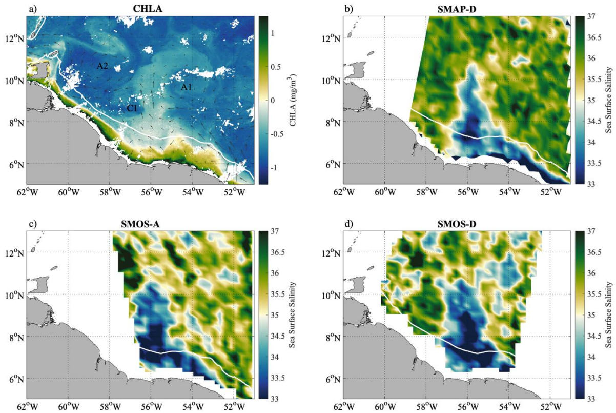
218 219 Figure 3: Satellite maps on February 12 th . Chla and geostrophic currents (grey arrows, a), 220 SMAP SSS along its descending track (b), SMOS SSS along its ascending (c) and descending 221 track (d) for the 12 th of February. The shelf break is represented by the 100-m bathymetry 222 contour (white line). Two anticyclonic (A1, A2) and one cyclonic (C1) eddy are labelled in 223 (a).
