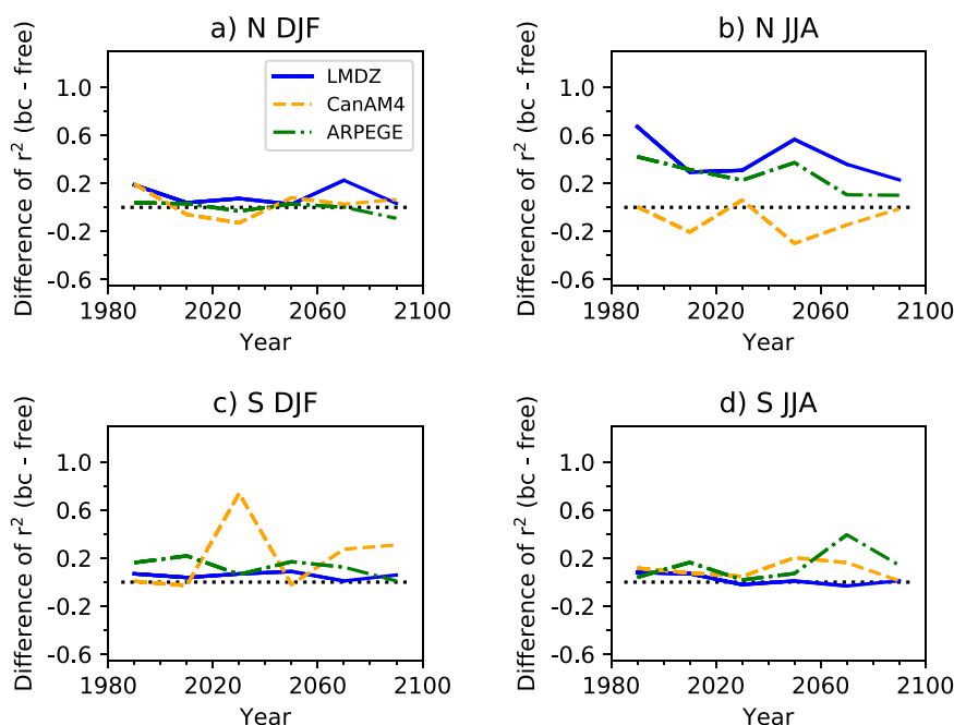
Fig. 3 Interannual variability of extratropical circulation. Squared spatial correlation coefficient ( r^2 ) of the first EOF of monthly mean extratropical (polewards of 30^\circ\text{N} and S) 500 hPa geopotential (20-year periods), bias-corrected minus uncorrected simulation. a Northern hemisphere winter (DJF); b Northern hemisphere summer (JJA); c Southern hemisphere winter (DJF); d Southern hemisphere summer (JJA).
