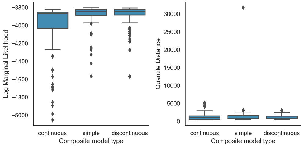
Figure 5: Log marginal likelihood and quantile distance of the fitted composite models depending on their type.
