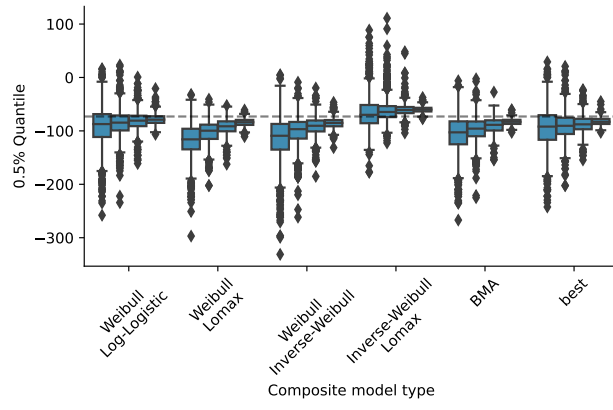
(c) 0.05% quantile
