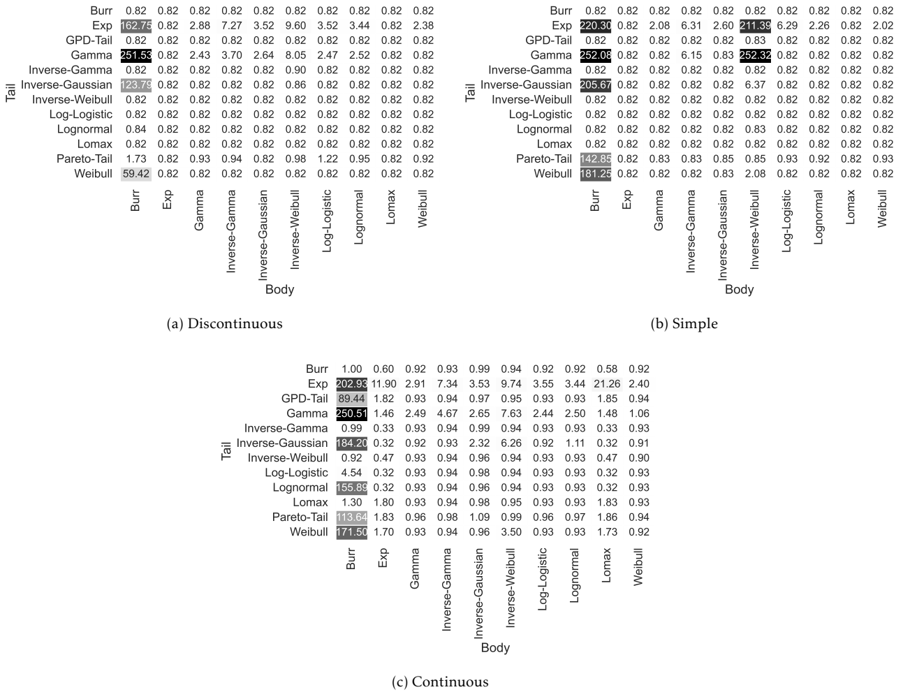
Figure 7: Posterior mean of the threshold resulting from the simultaneous estimation of the composite model parameters.
