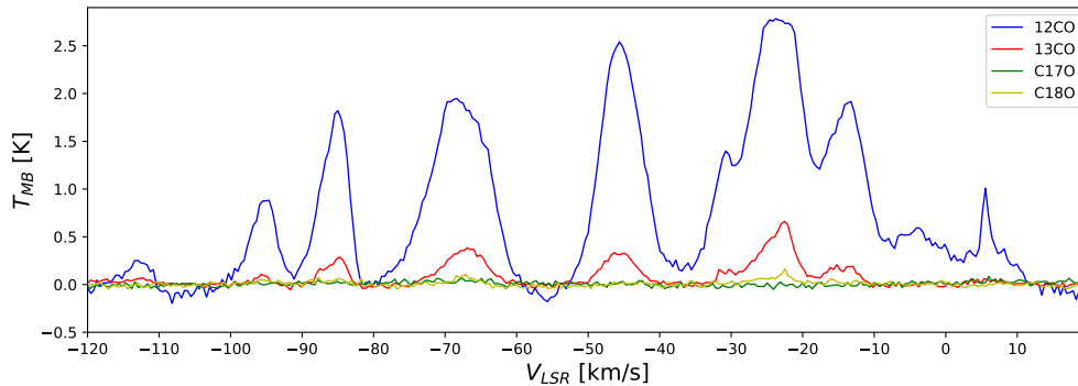
Fig. H.3. Brightness temperature peaks obtained by integrating the data from the Mopra radio survey (Braiding et al. 2018) within a 0.3°-side square window centered at the best-fit position of HESS J1702-420A (shown in red in Fig. H.4).
