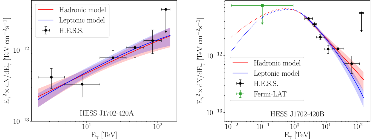
Fig. 5. Models of \gamma -ray emission based on hadronic (red) and leptonic (blue) one-zone scenarios, for HESS J1702-420A – left panel – and HESS J1702-420B – right panel . The best-fit spectra, under the assumption of simple power law distribution of the underlying particle populations, are shown as solid lines, while the shaded areas and dotted lines represent the 1\sigma statistical error envelope and extrapolations outside the fit range, respectively. The H.E.S.S. and Fermi -LAT flux points are also shown, for reference purpose. Fit results were obtained with a 3D fit of H.E.S.S. data.
