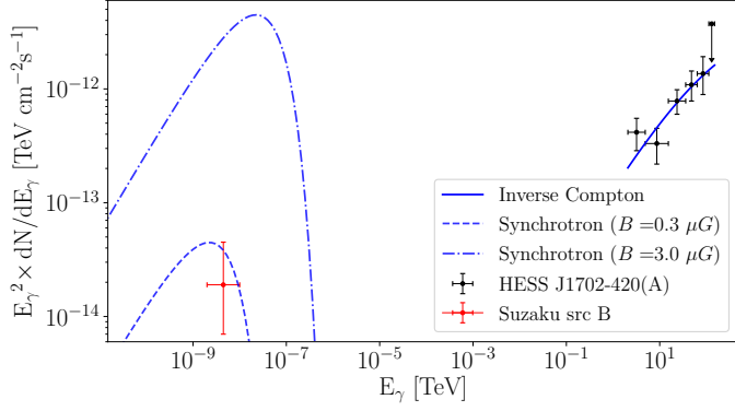
Fig. H.5. multi wavelength modeling of HESS J1702-420A, under the assumption of a one-zone leptonic scenario powered by a power law distribution of electrons. The synchrotron emission was computed assuming a magnetic field value of 0.3 and 3 \mu G. The black error bars represent the VHE flux points of HESS J1702-420A, while the red one indicates the flux of the unidentified Suzaku src B (Fujinaga et al. 2011).
