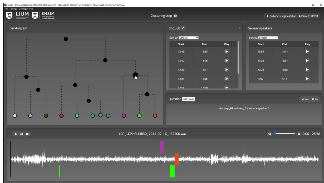
Figure 1: Screenshot of the graphical user interface of the LIUM Human Active Correction Platform for speaker diarization.
