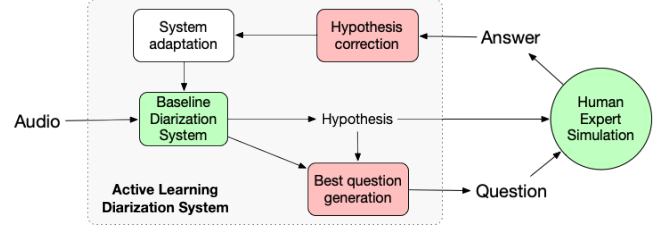
Figure 1: Life-cycle of a human assisted speaker diarization system.
