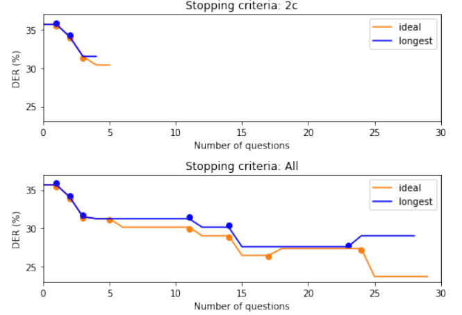
Figure 3: Tracking of the DER corresponding to a single show file (with duration of 1 hour and 11 minutes) by applying question-correction with different methods. Points in each question indicate that it has resulted in a correction.
