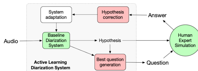
Figure 1: Life-cycle of a human assisted speaker diarization system.
