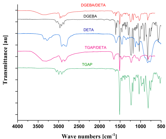
Fig. 2. FTIR spectra of the DETA hardener, DGEBA and TGAP resins, and the DGEBA/DETA and TGAP/DETA polymers.
