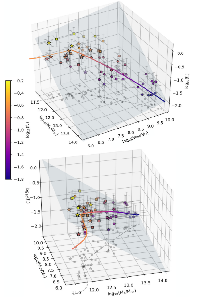
Figure 3. Two different 3D views for the distribution of our galaxy sample in the ( M_{\text{h}} , M_{\text{BH}} , f_{\star} ) space. The markers used in both panels are the same as in Fig. 1. The best-fitting plane from equation (1) is shown in dark grey. The 3D curve passing through the data shows the fiducial theoretical model from Section 4. To better enhance the 3D perspective, galaxies are colour-coded by their f_{\star} and 2D projections on the ( M_{\text{h}} , M_{\text{BH}} ) plane are shown.
