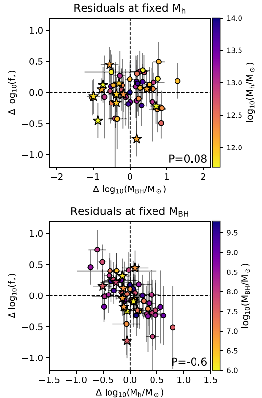
Figure 2. Top panel: residuals in the f_{\star}-M_{\text{h}} relation versus residuals in the M_{\text{BH}}-M_{\text{h}} relation for our galaxy sample. At fixed M_{\text{h}} , there is weak tendency for galaxies hosting heavier BHs to show larger f_{\star} (Pearson coefficient of 0.1). The colour palette shows the M_{\text{h}} of each galaxy. Bottom panel: residuals in the f_{\star}-M_{\text{BH}} relation versus those in the M_{\text{h}}-M_{\text{BH}} relation. At fixed M_{\text{BH}} , there is a strong evidence for galaxies living in lighter haloes to have larger f_{\star} (Pearson coefficient of -0.6 ). The colour palette shows the M_{\text{BH}} of each galaxy. The markers used in both panels are the same as in Fig. 1.
