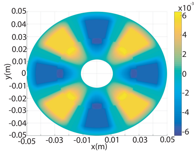
(a) i_a = 0 \text{ A} , i_b = 0 \text{ A} , i_c = 0 \text{ A} , B_r = 1.01 \text{ T} and \rho = 0^\circ
