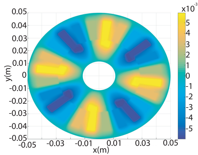
(c) i_a = 0 \text{ A} , i_b = 0 \text{ A} , i_c = 0 \text{ A} , B_r = 1.01 \text{ T} and \rho = 10^\circ
