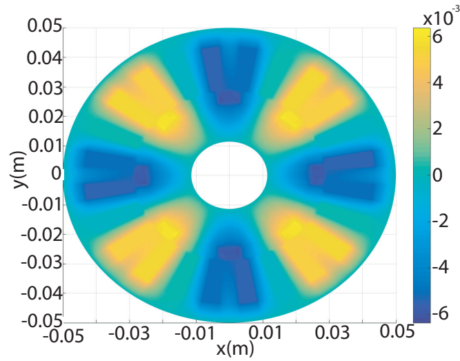
(b) i_a = -1.5 \text{ A} , i_b = 3 \text{ A} , i_c = -1.5 \text{ A} , B_r = 1.01 \text{ T} and \rho = 0^\circ
