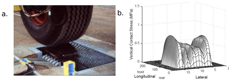
Figure 1. a. Set of instrumented tips; b. Distribution of contact pressures measured under a tire by this experimental assembly [5]
