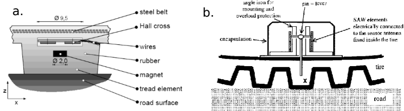
Figure 4. Instrumented tread block: a. Hall effect [9] ; b. SAW sensors [10]
