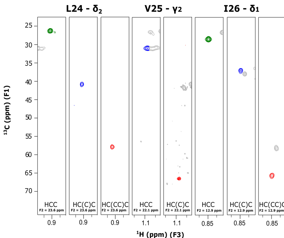
1 2 3 Fig. S2 Application to the 87 kDa prefoldin from Pyrococcus horikoshii . Examples of 2D- 4 extracts from 3D ‘out and back’ HCC , HC(C)C and HC(CC)C experiments correlating ^1\text{H} (F 3 ) 5 and ^{13}\text{C} (F 2 ) methyl resonances with ^{13}\text{C}_\gamma (green) ^{13}\text{C}_\beta (blue) or ^{13}\text{C}_\alpha (red) in F 1 dimension of 6 Leu-24, Val-25 and Ile-26 of Pyrococcus horikoshii prefoldin subunit \beta . Spectra have been 7 recorded at 310 K using 0.2 mM U- ^{2}\text{H} , ^{15}\text{N} , ^{13}\text{C} ], Ile-[2, 3, 4, 4- ^2\text{H}_4 ; 1, 2, 3, 4- ^{13}\text{C}_4 ; 8 ^{13}\text{C}^1\text{H}_3 ] ^{\delta 1} /[ ^{12}\text{C}^2\text{H}_3 ] ^{\gamma 2} ], Leu-[2, 3, 3, 4- ^2\text{H}_4 ; 1, 2, 3, 4- ^{13}\text{C}_4 ; [ ^{13}\text{C}^1\text{H}_3 ] ^{\text{pro-S}} /[ ^{12}\text{C}^2\text{H}_3 ] ^{\text{pro-R}} ], Val-[2, 3- 9 ^2\text{H}_2 ; 1, 2, 3- ^{13}\text{C}_3 ; [ ^{13}\text{C}^1\text{H}_3 ] ^{\text{pro-S}} /[ ^{12}\text{C}^2\text{H}_3 ] ^{\text{pro-R}} ] sample of prefoldin on an NMR spectrometer 10 operating at a proton frequency of 950 MHz. The acquisition parameters were similar to that 11 used for HSP90-NTD, described in Materials and Methods section. Prefoldin was expressed 12 and purified according to the protocol described in Törner et al. (2020) and labelled on the \beta 13 subunit only using labelling scheme A, described in Materials and Methods section of the 14 present manuscript.
