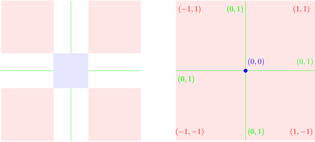
Figure 1: In this figure \text{pen}(b) = |b_1| + |b_2| . On the left the blue polytope is B^* = \partial_{\text{pen}}(0) = \text{conv}\{\pm(1,1), \pm(1,-1)\} ( B^* is the unit ball of the \ell_\infty norm). Red and green (unbounded) sets are preimages, with respect to the projection onto B^* , of vertices and edge centers. The picture on the right provides \text{sign}(x) \in \{(0,0), \pm(1,0), \pm(0,1), \pm(1,1), \pm(1,-1)\} depending on the localization of x \in \mathbb{R}^2 .
