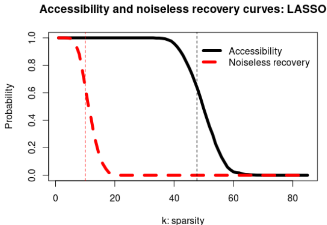
Figure 7: These curves provide the probability of the noiseless recovery condition and the probability of the accessibility condition as functions of the support size k . The value k = 50/\log(150) = 9.9 (Wainwright, 2009) is, approximately, the preimage of 0.5 for the noiseless recovery curve and k = 100\rho_{DT}(2/3) = 47.8 , where \rho_{DT} is the phase transition curve (Donoho and Tanner, 2009b,a), is approximately the preimage of 0.5 for the accessibility curve.
