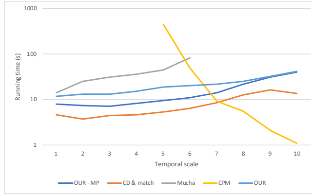
Fig. 3: Speed of several dynamic community detection methods for several temporal granularities, on the Math Overflow dataset. Missing points correspond to computation time above 1000s. Temporal scales correspond to window sizes and are divided by 2 at every level, from 1=67 681 200s (about 2 years) to 10=132 189s (about 36h). OUR and OUR-MP corresponds to our method using or not multiprocessing (4 cores)
