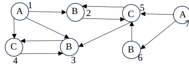
Fig. 3: Match graph G_s
