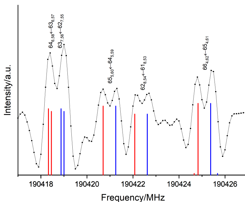
Figure 7. Tunnelling splittings observed in the pure rotational mm-wave spectrum within the |v_{35} = 1\rangle ES. Each doublet associated with J''_{K''_a, K''_c} \leftarrow J''_{K''_a, K''_c} rotational transitions represented by their blue and red components.
