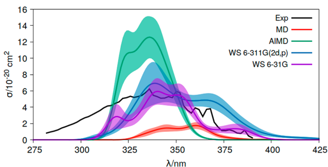
Figure 2. Absorption cross sections ( \sigma ) of acrolein in the gas phase measured experimentally (Exp) 55,57 and computed at the CASPT2-(6,5)/ANO-L-VTZP level of theory using distinct conformational sampling approaches, classical molecular dynamics (MD), ab initio molecular dynamics (AIMD), and Wigner sampling (WS). For WS, two basis sets are compared, 6-31G (WS 6-31G) and 6-311G(2d,p) (WS 6-311G(2d,p)). Shadow areas represent the statistical error of the approach ( \delta\sigma(E) ).
