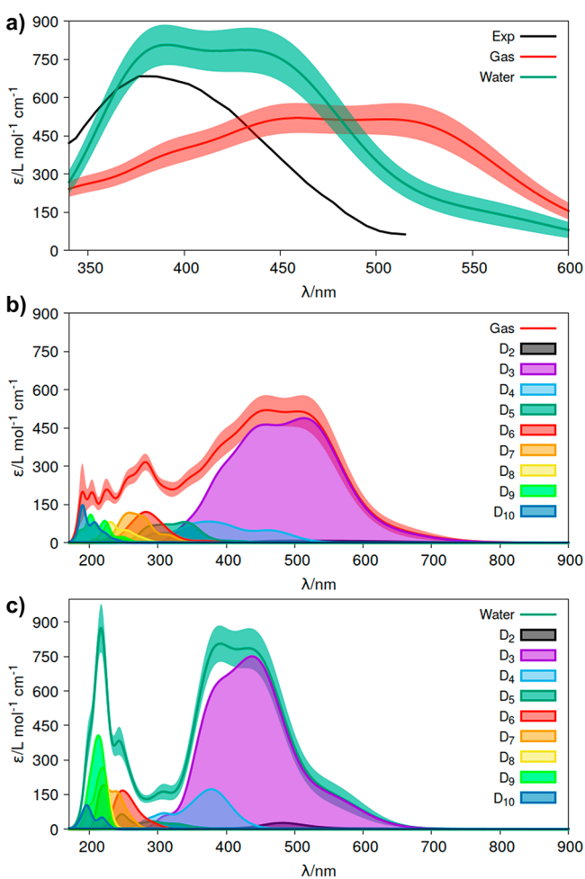
Figure 6. (a) Absorption molar extinction coefficients ( \epsilon ) of the radical formed upon attachment of an OH radical at the C6 position of the uracil molecule ( U6OH^{\bullet} ) computed in the gas phase and in a water solution and absorption spectra of the transient species produced 67 experimentally in an aqueous medium after water radiolysis in the presence of the uracil nucleobase. Shadow areas represent the statistical error of the approach ( \delta\epsilon(E) ). (b) Deconvolution of the absorption spectrum in the gas phase related to the electronic transitions between the ground state of the system ( D_1 ) and the excited states ( D_2 – D_{10} ). (c) Analogous deconvolution of the spectrum in water.
