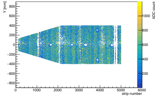
Figure 50: Cluster charge on Module 11 Layer 2 for all PCBs. 5 PCBs give 4 thin vertical gaps due to the passivation over the borders of PCBs. The empty gaps in addition to the interconnections and PCB borders (around strip number 4800) are caused by bad connections of electronics.
