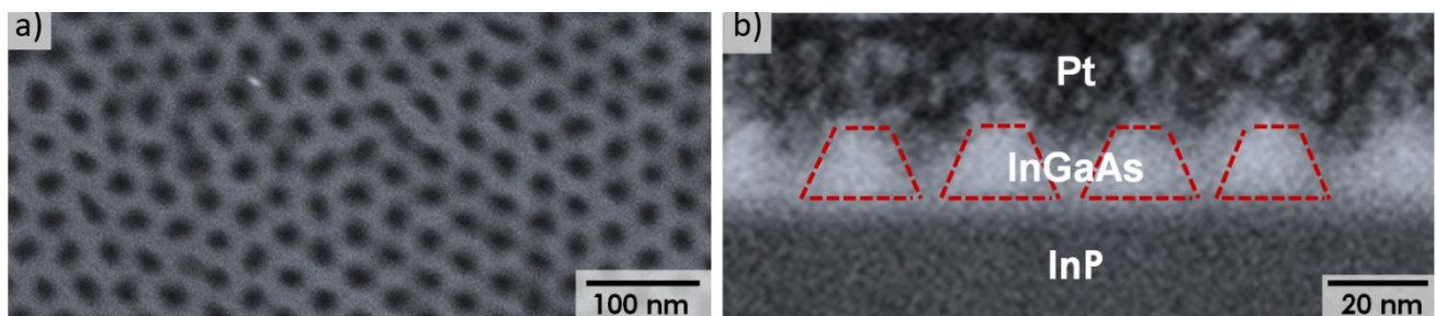
Fig. 3: a) SEM and b) cross-sectional TEM images of the honeycomb \text{In}_{0.53}\text{Ga}_{0.47}\text{As} quantum well nanoporated
