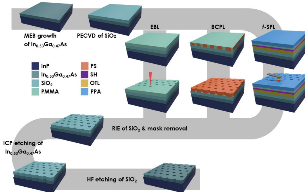
Fig. 1: Schematic workflow diagram for lithographic fabrication of a triangular antidot lattice in an \text{In}_{0.53}\text{Ga}_{0.47}\text{As} quantum well grown on a \text{InP} (001) substrate by molecular beam epitaxy (MBE). Three techniques were used: e-beam lithography (EBL), block copolymer lithography (BCPL) and thermal scanning probe lithography (t-SPL).
