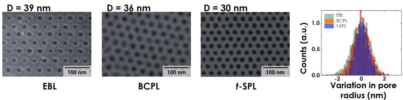
Fig. 2: SEM images of the masks prepared with EBL, BCPL and t-SPL. The periodicity of the triangular lattice is indicated for each mask. Comparison of the pore size variation for the three different masks.
