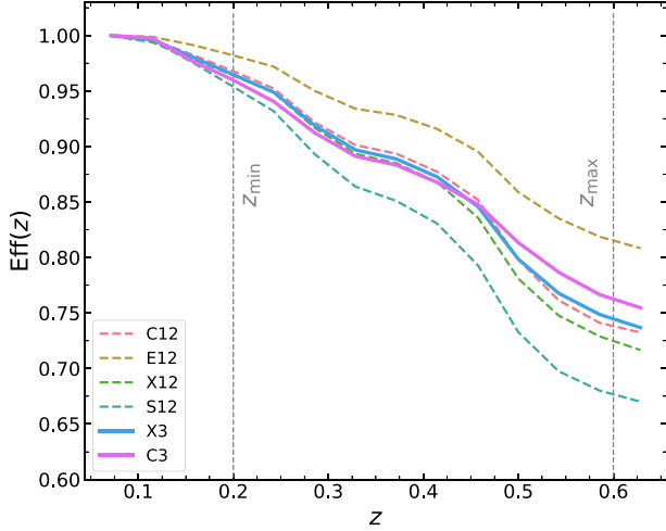
Figure 3. SN host galaxy spectroscopic efficiencies as a function of redshift z . Efficiency curves are grouped by shallow ( \{F\}12 ) and deep ( \{F\}3 ) fields, and averaged over the 5 yr of the survey. The lower and upper redshift limits for this analysis are indicated by z_{\min} and z_{\max} , respectively.
