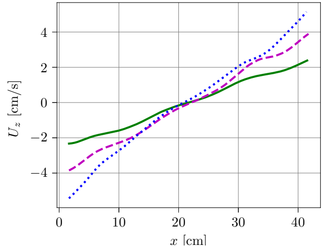
Fig. 4: Velocity profiles at mid-height in the \Gamma = 1 cell with FC770 as the working fluid. Solid green line: Ra = 3.6 \times 10^{11} , dashed purple line: Ra = 9.7 \times 10^{11} , dotted blue line: Ra = 2.1 \times 10^{12} .
