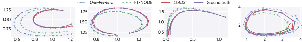
Figure 3: Test prediction obtained with two baselines ( One-Per-Env. and FT-NODE) and LEADS compared with ground truth for LV in phase space for 4 envs., one per figure from left to right.
