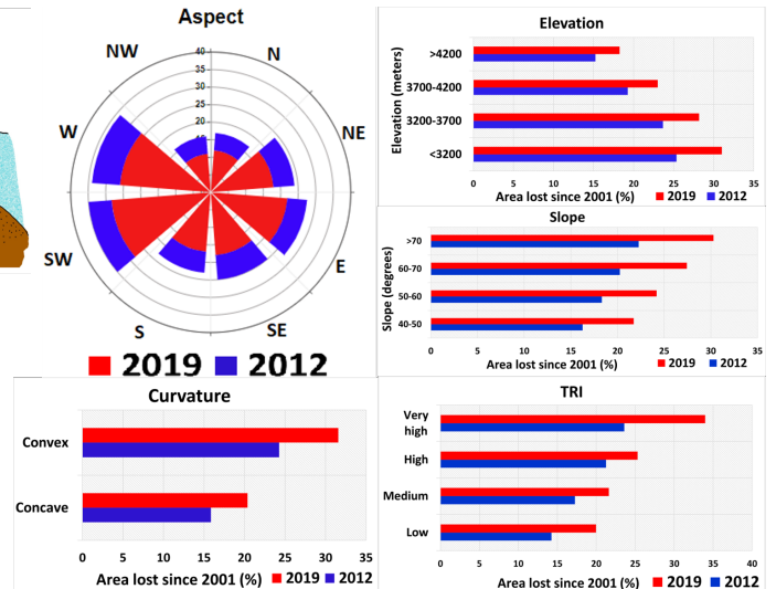
Figure 2. Influence of topographic factors on relative area loss of Ice Aprons in the Mont Blanc Massif
