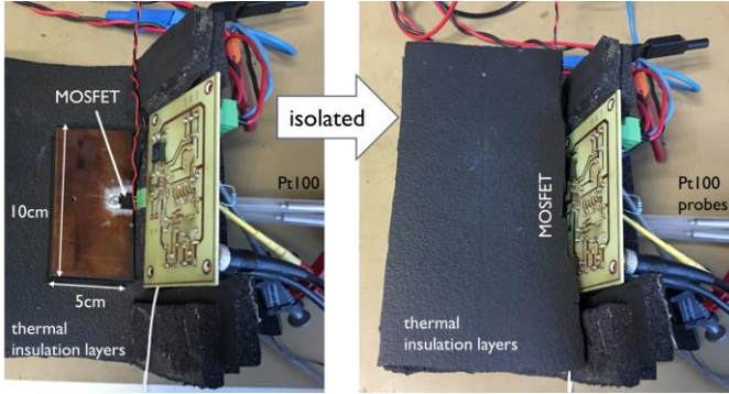
Fig. 9. Test bench
